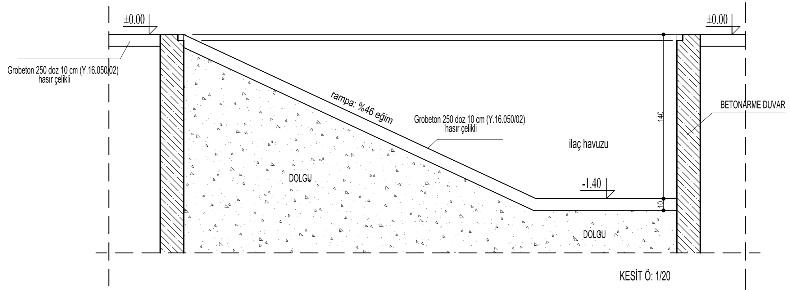
SAC KAPAK PLANI Ç:1/20
